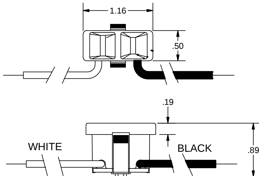
438 With 6" lg. Wire Leads
