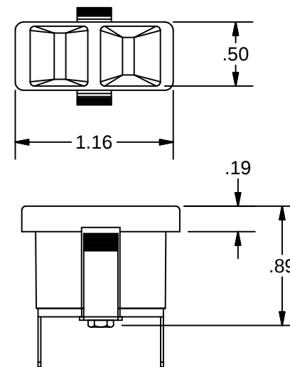
438-M With Male Tabs
